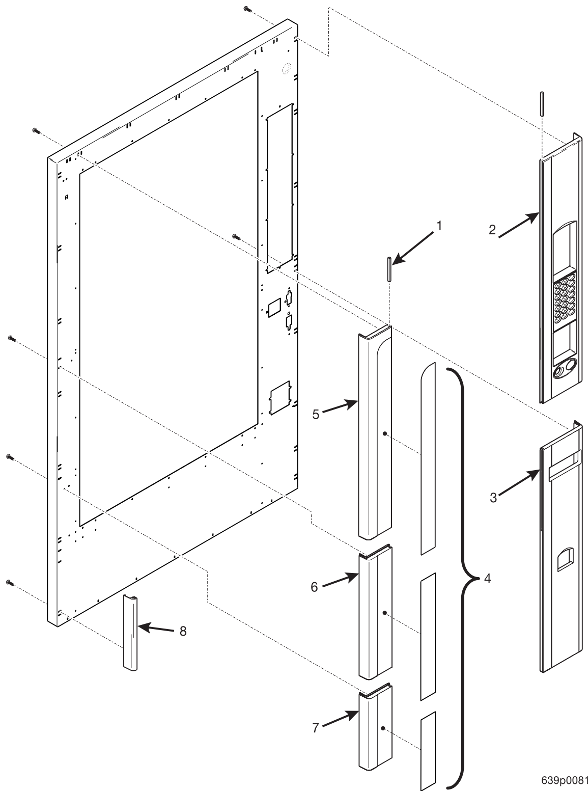
Figure 3. Millennium Trim - Part 1
