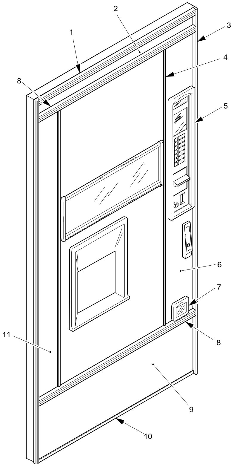
Figure 2. Trim - Standard Style
