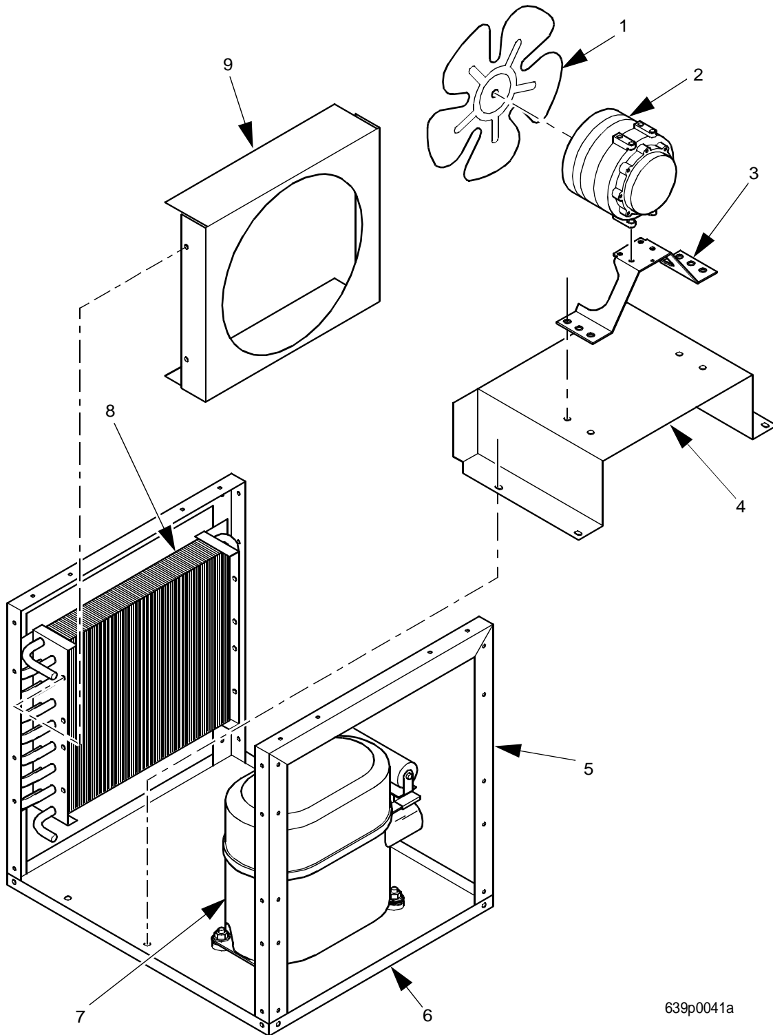
Figure 78. Condensing Unit Detail
