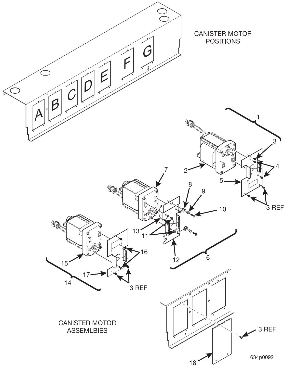
Figure 74. Canister Motor Options and Assemblies
