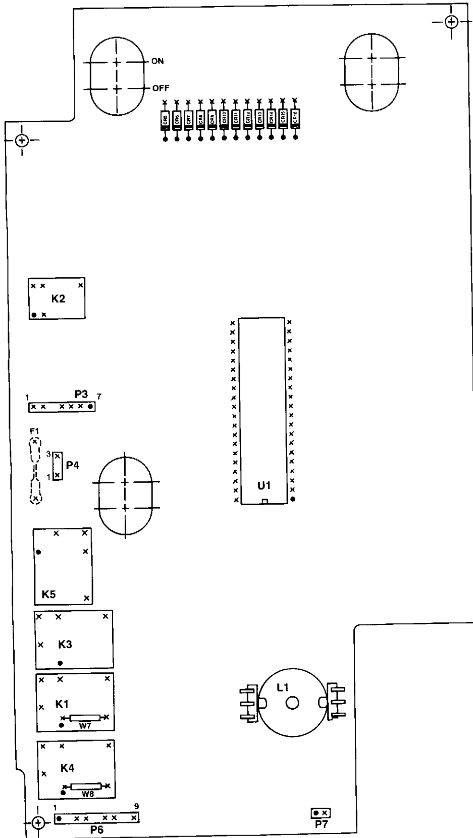
Figure 5.1 Logic Board Partial Layout
