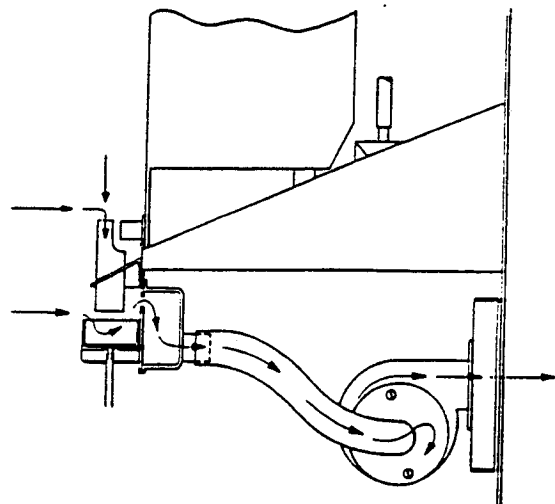
STEAM EXHAUST FLOW
