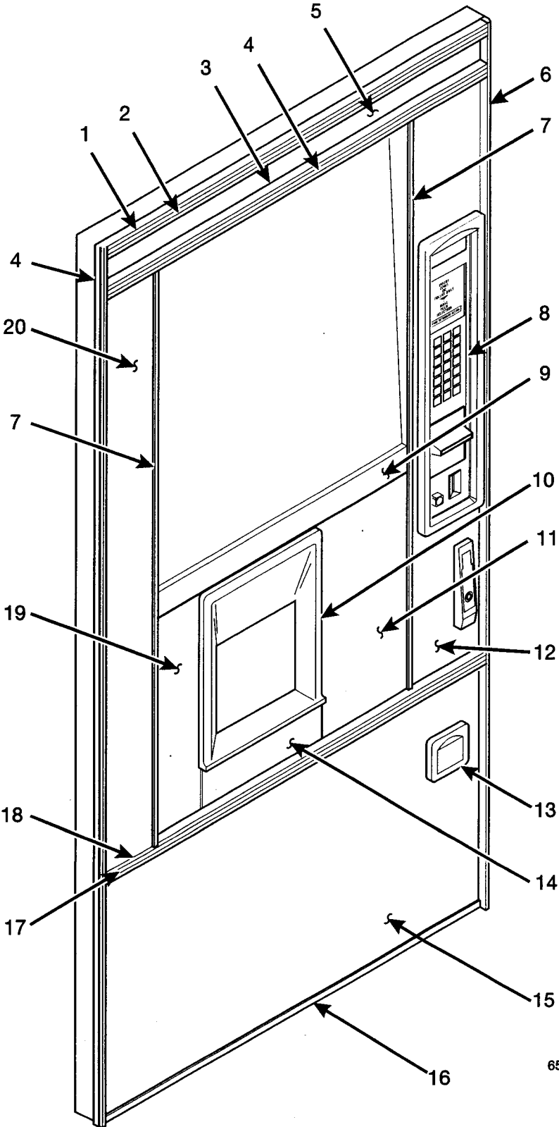
Figure 2. Trim Components
